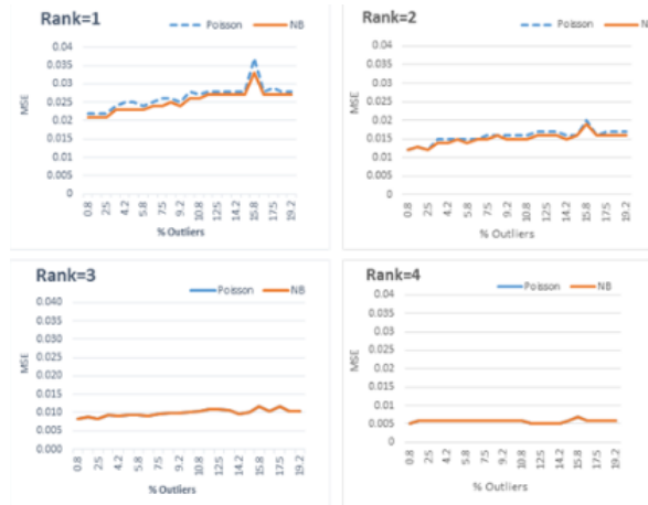
Figure 3: The MSE of RCIM rank=1, 2, 3 and 4 for Poisson and Negative Binomial (NB) Distributions on Simulated Data containing 0.8% - 19.2% outliers
